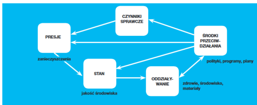
Ryc. 1. Model D-P-S-I-R
